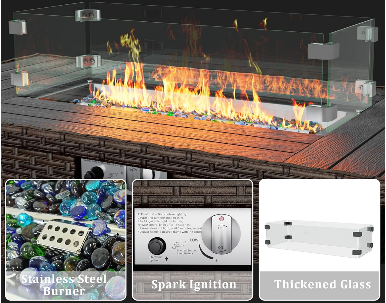
Image: Detailed view of the fire pit's components, including the 50,000 BTU burner, spark ignition mechanism, and the protective thickened glass wind guard.
