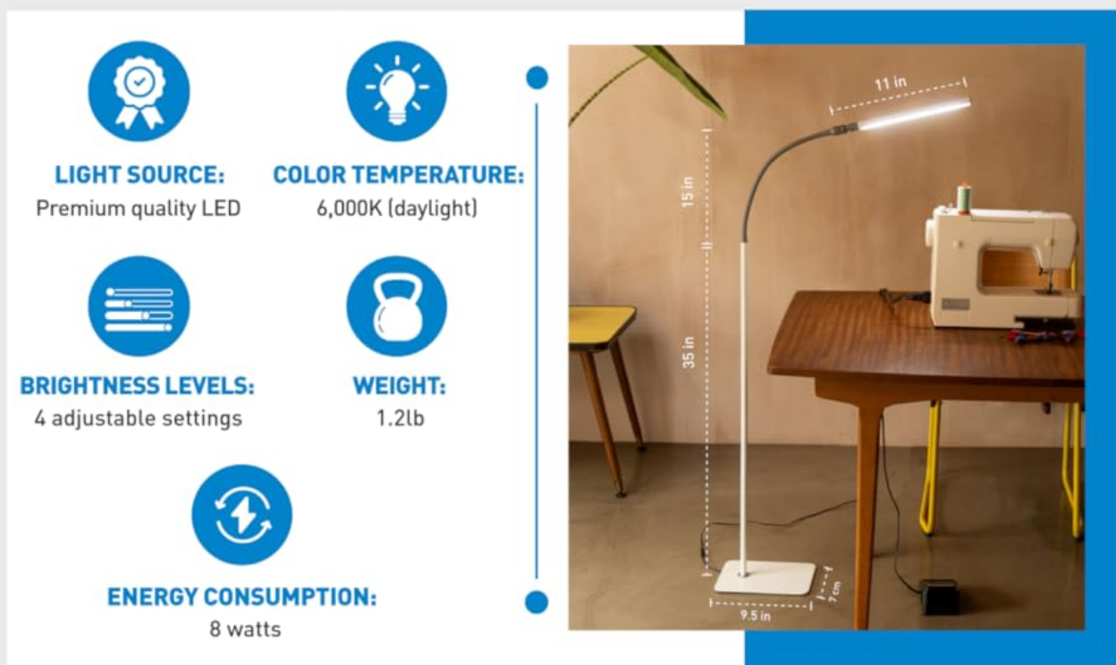
Figure 4: Lamp adjustability features.
