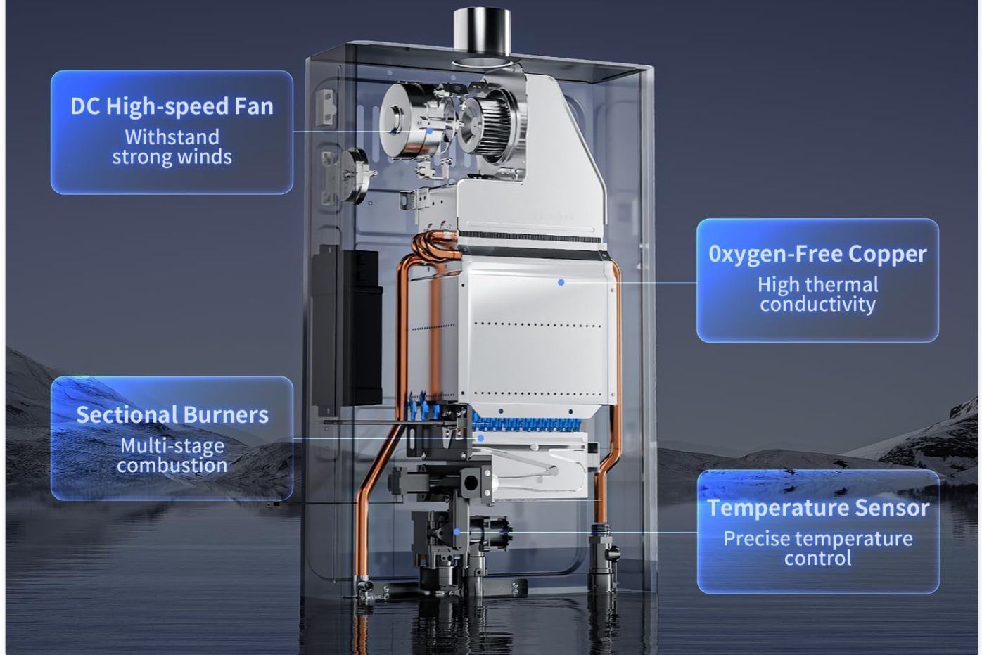
Figure 4: Detailed view of the HeatMaster 2.0 Water Heating System, highlighting the DC High-speed Fan, Oxygen-Free Copper, Sectional Burners, and Temperature Sensor.
