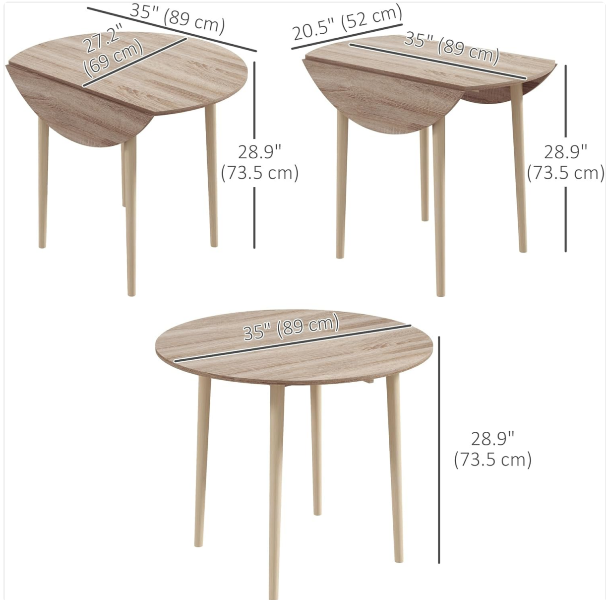
Image 7.1: Dimensional diagram illustrating the table's size when fully extended (35" Dia. x 28.9" H), with one leaf folded (35" L x 27.2" W x 28.9" H), and with both leaves folded (35" L x 20.5" W x 28.9" H).
