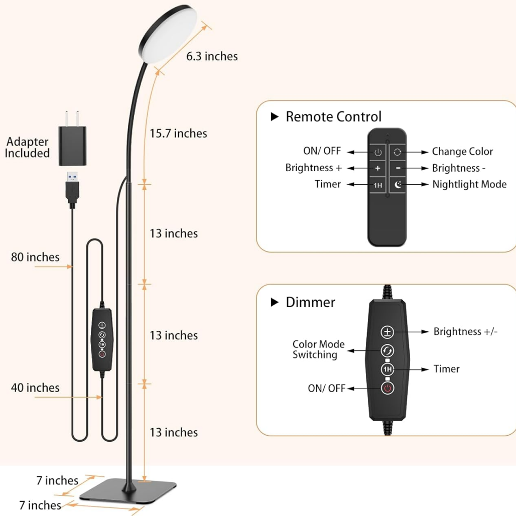
Image: Diagram showing the dimensions of the Mojimdo LED Floor Lamp, including the lamp head diameter, gooseneck length, pole section lengths, base dimensions, and cable length. Also details the remote control and dimmer functions.
