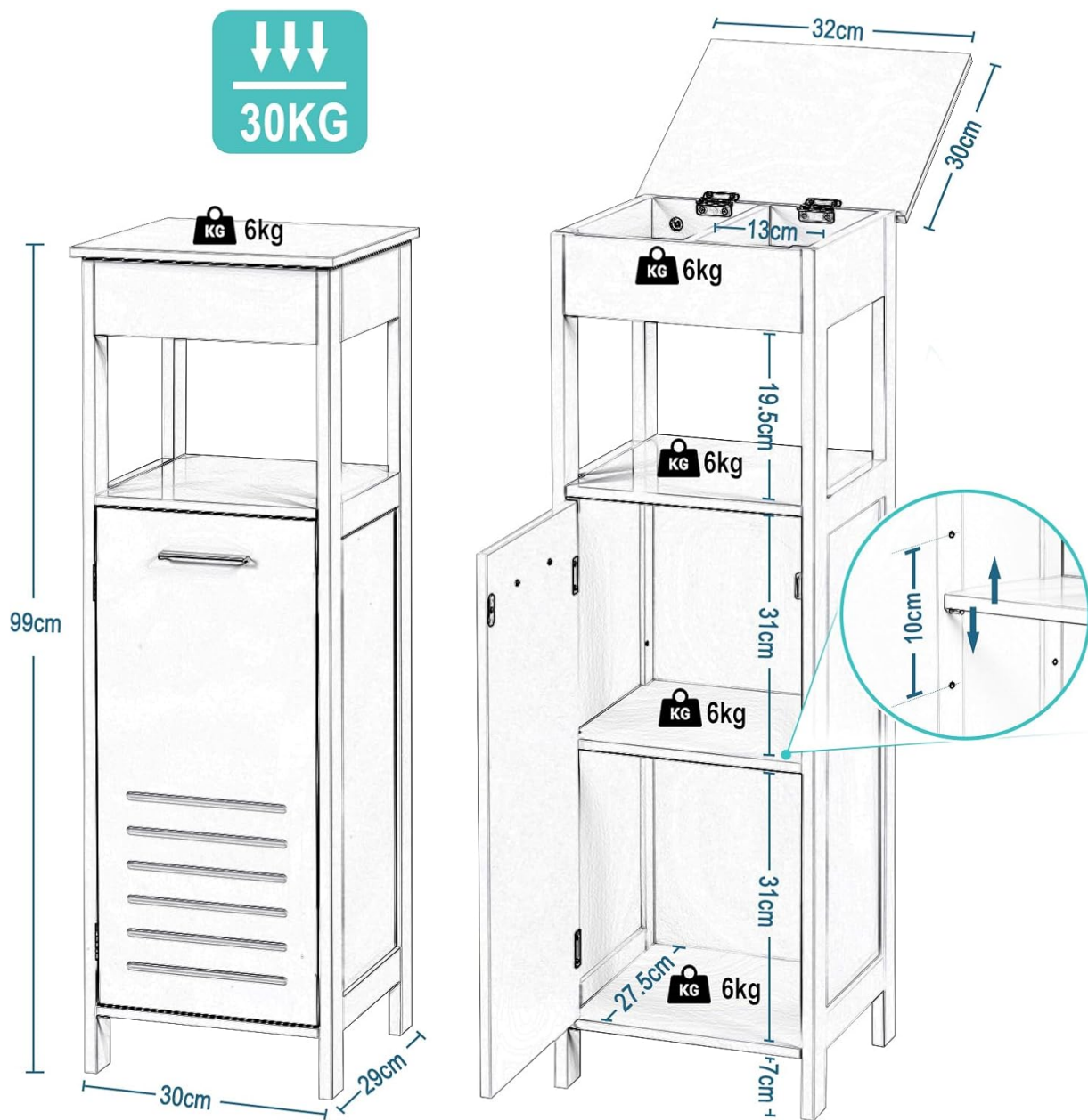
Image: Cabinet dimensions and internal structure for assembly reference.
