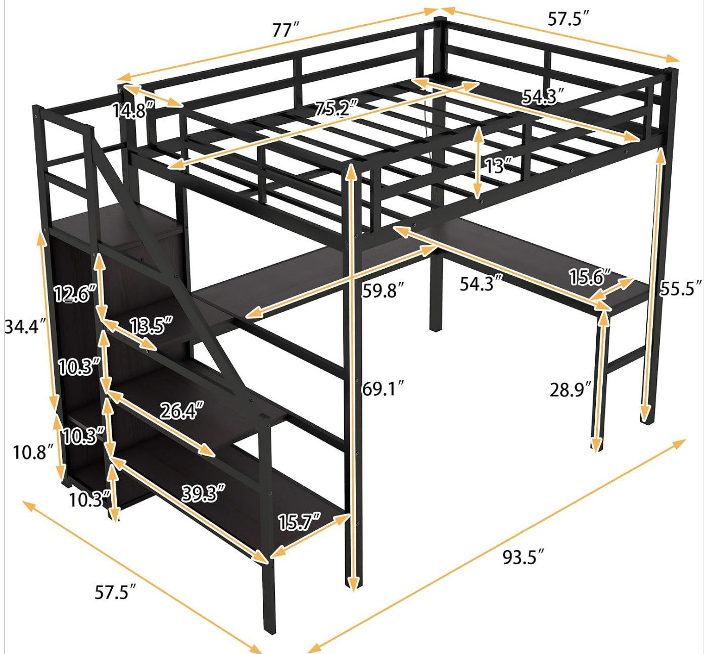
Image: Detailed dimensions of the Bellemave Full Size Loft Bed, showing overall length, width, and height, as well as desk and stair measurements.
