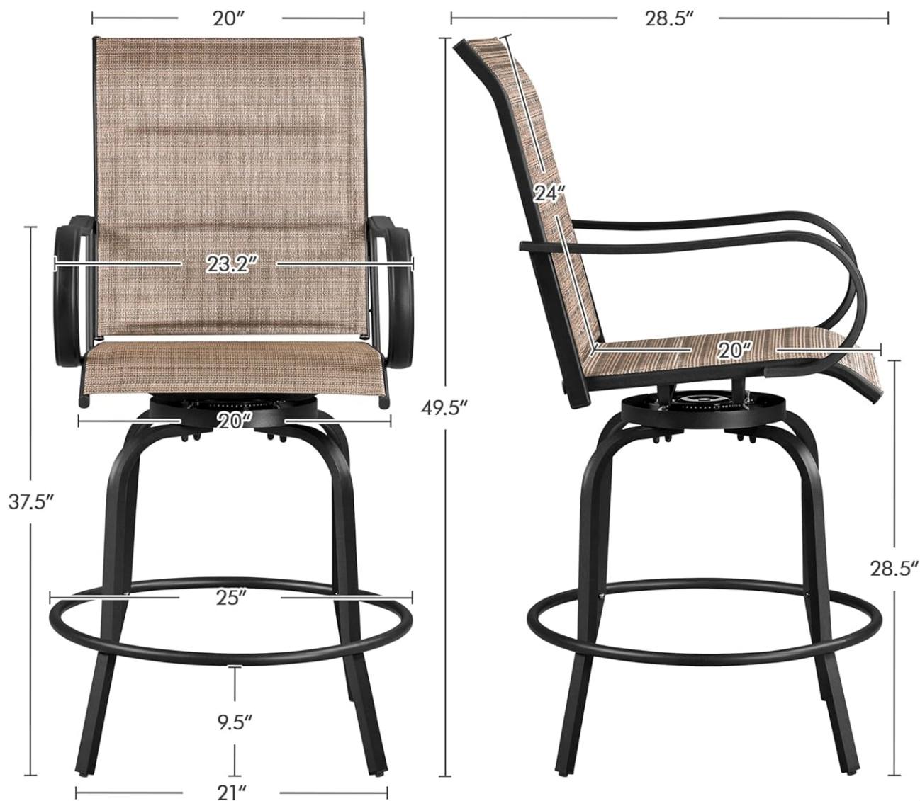
Figure 6: Detailed dimensions of the bar stool.
