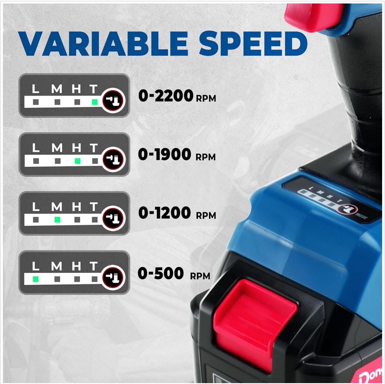
Figure 5: Variable speed and torque settings.
