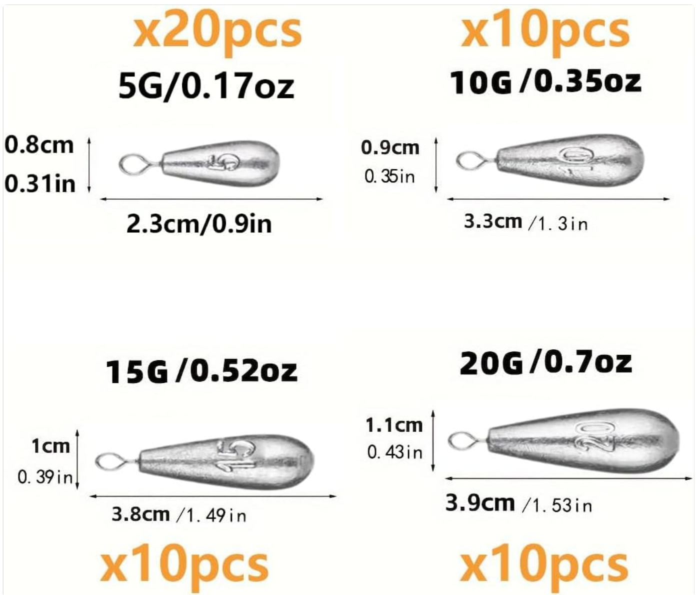
Image: Detailed dimensions for each sinker weight (5g, 10g, 15g, 20g).
