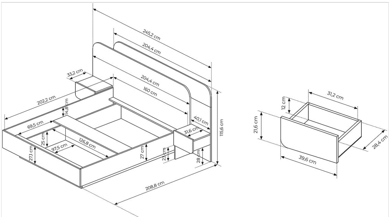
Image 4.1: Assembly diagram with key dimensions for the DESADO bed and its integrated nightstand drawers.
