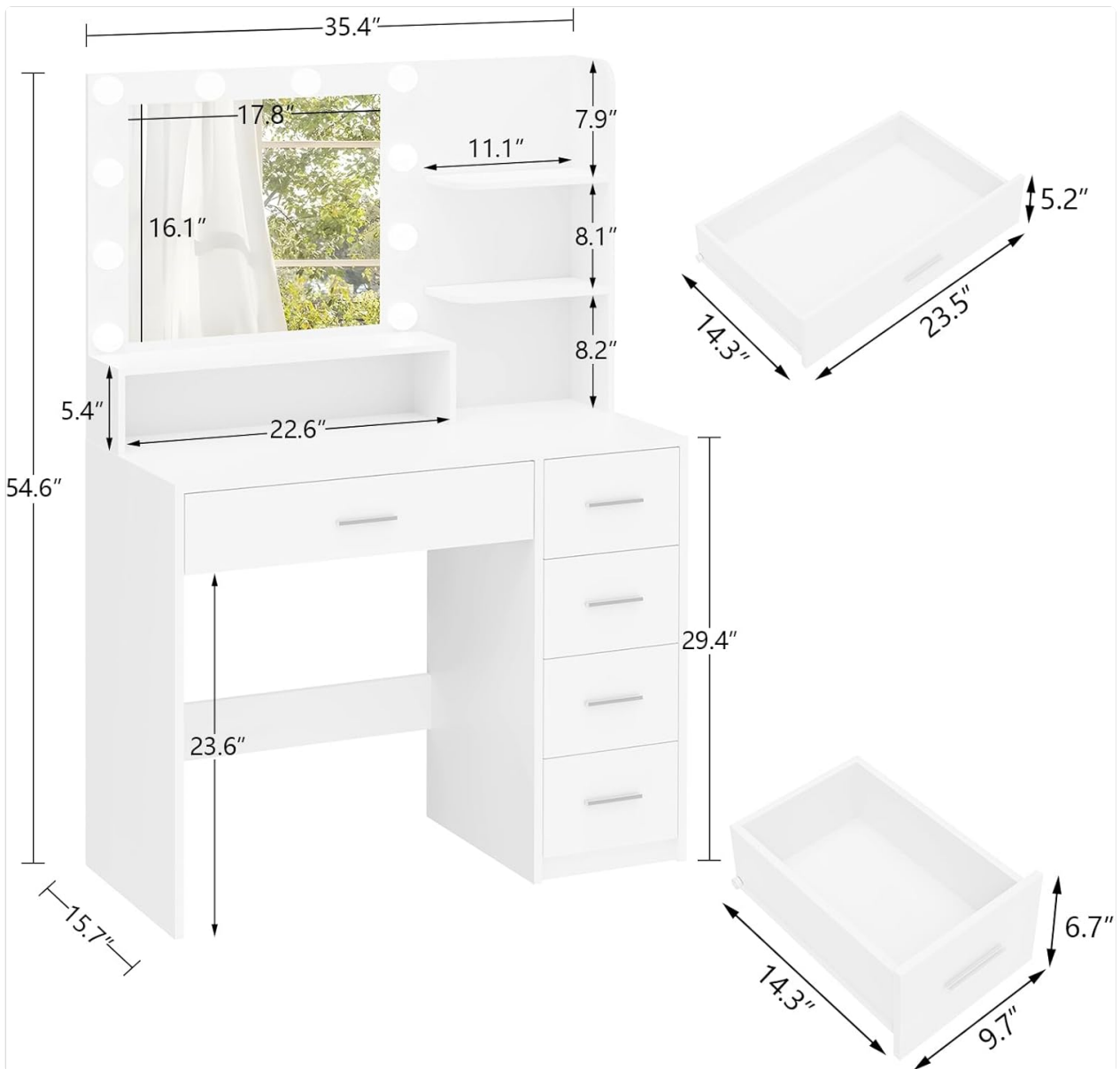
Figure 5: Drawer Details
