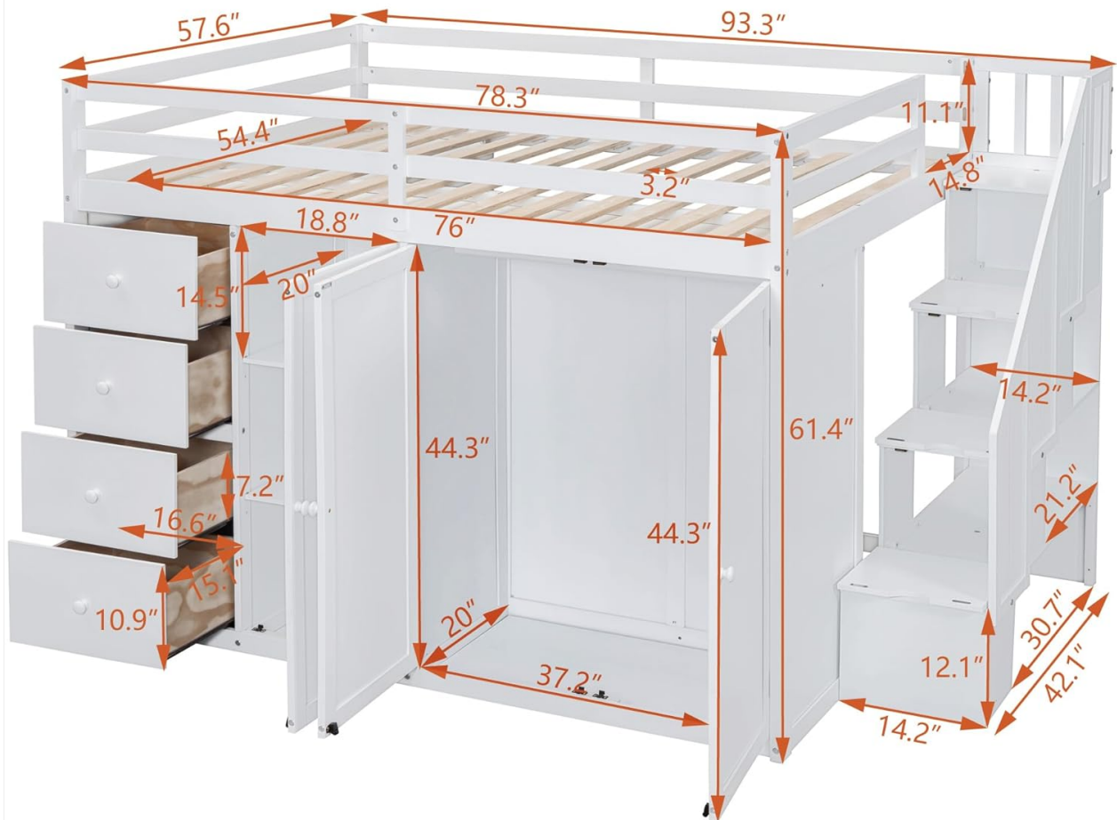
Image: Detailed dimensions of the Merax Full Size Loft Bed, showing length, width, and height measurements for all components in inches.
