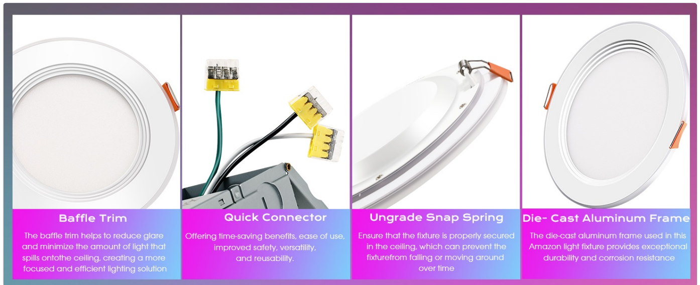
Figure 4: Initial setup process for smart light connectivity.
