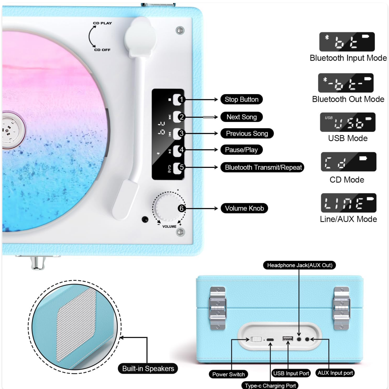
Figure 3: Control Panel and Port Layout.
