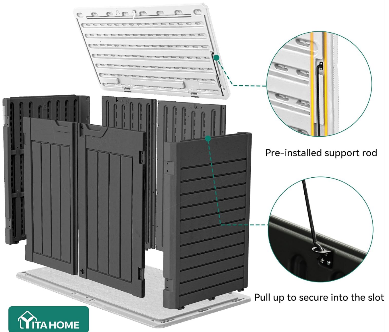
Figure 3.1: Easy Assembly and Disassembly Overview
