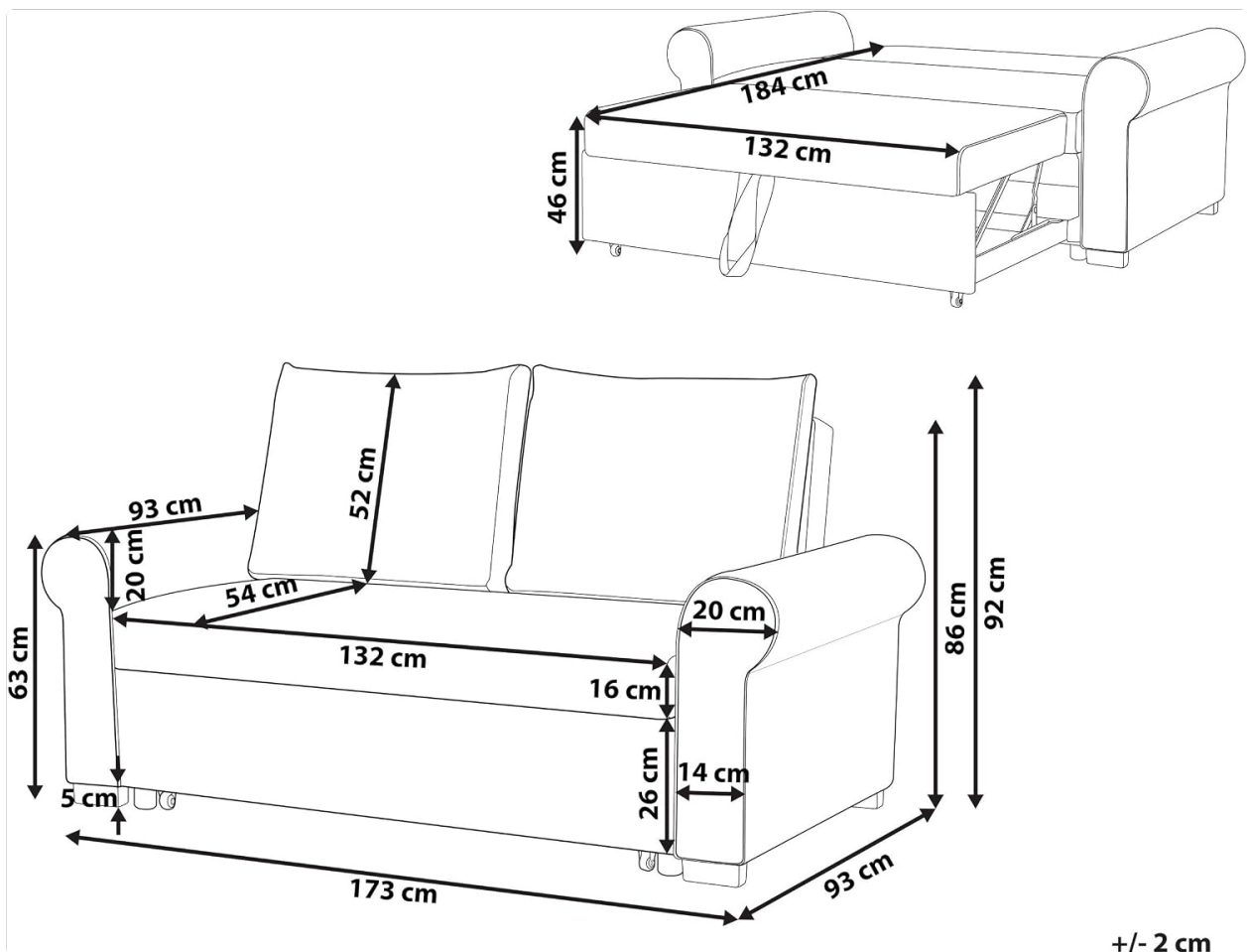
Image: A technical diagram illustrating the dimensions of the Beliani Silda Retro Pull-Out Sofa Bed in both sofa and extended bed configurations, with measurements in centimeters.
