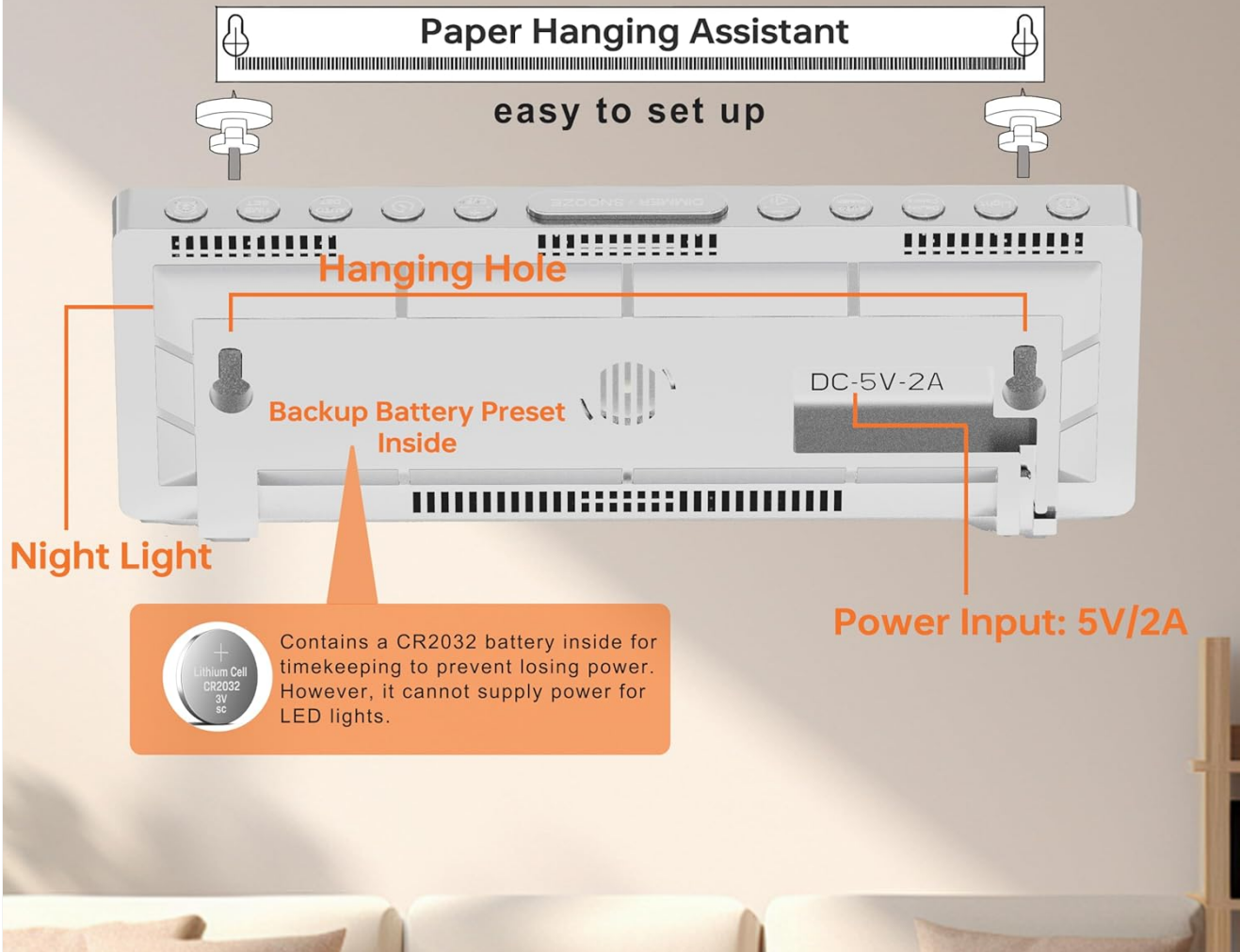
Figure 3: The back of the JALL Digital Alarm Clock, highlighting the DC 5V-2A power input, the integrated hanging holes for wall mounting, and the location of the internal memory battery.
