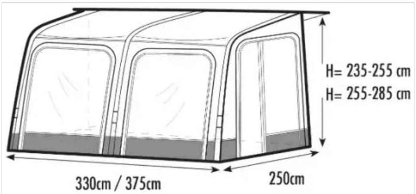
Image: Technical diagram showing the dimensions of the Westfield Vega 375 2.0 awning.
