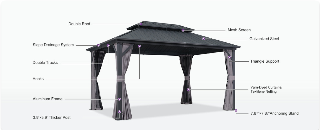
Image: Visual representation of key gazebo features such as the water gutter, triangle support, anchoring stand, ceiling hooks for lights, yarn-dyed curtains, and textile netting.
