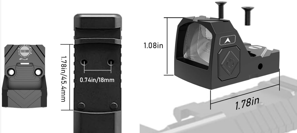
Image 6.1: Product dimensions.
