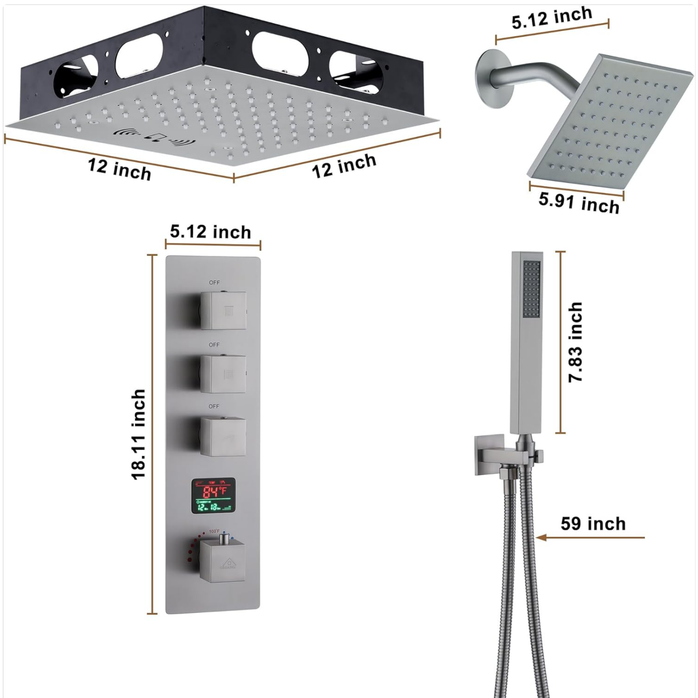
Figure 2: Product Dimensions - Detailed measurements for the shower heads, control panel, and handheld spray.
