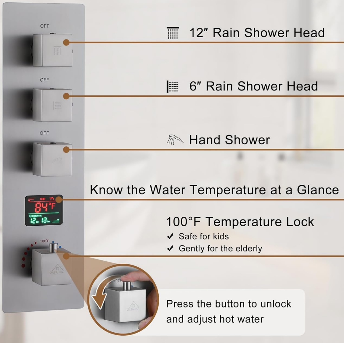
Figure 4: Temperature Control - Illustrates the temperature display and safety lock feature.
