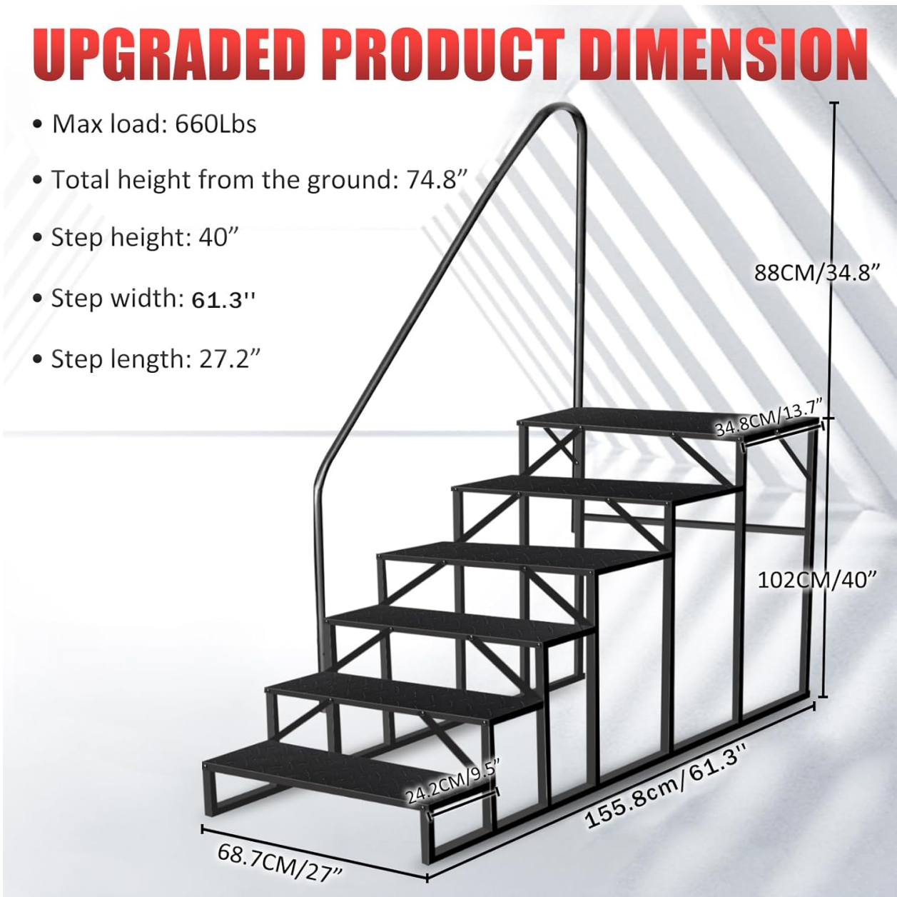
Detailed dimensions of the RV steps, including max load, total height, step height, width, and length.
