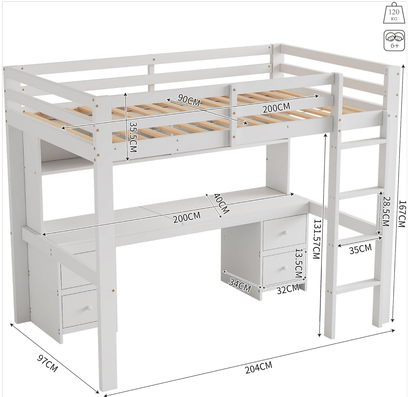
Figure 3.1: Diagram showing the dimensions of the Moimhear Loft Bed, including bed, desk, and storage measurements. This image can be used as a reference during assembly.
