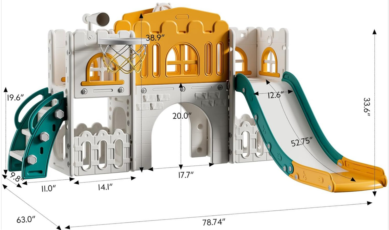
Image 2.2: Detailed product dimensions of the playset, showing overall length, width, and height, as well as specific measurements for the slide and climbing areas.
