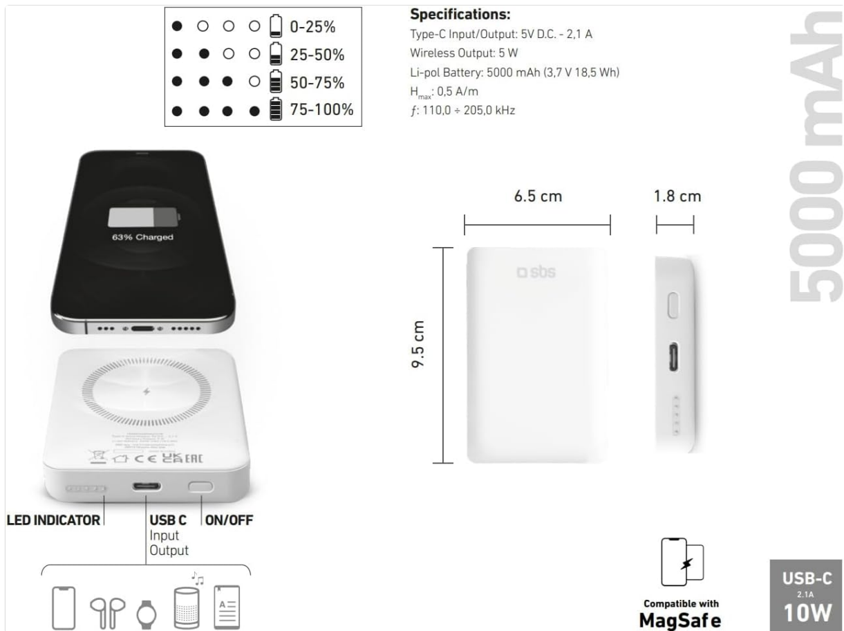
Image: A detailed diagram of the power bank, showing its dimensions (9.5 cm length, 6.5 cm width, 1.8 cm thickness), LED indicator guide for charge levels, and key specifications like USB-C input/output and wireless output.
