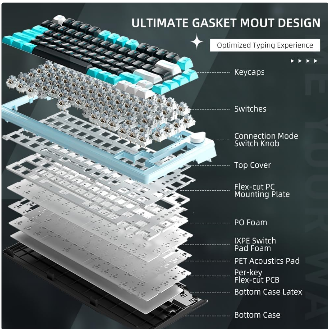
Image 2.2: Exploded view illustrating the multi-layered gasket mount design for enhanced typing feel.
