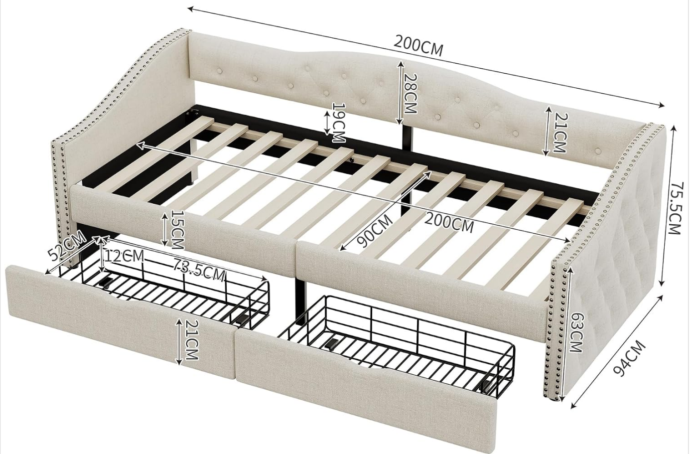
Figure 3.1: Dimensional diagram of the Moimhear Daybed, illustrating overall measurements and key component sizes.
