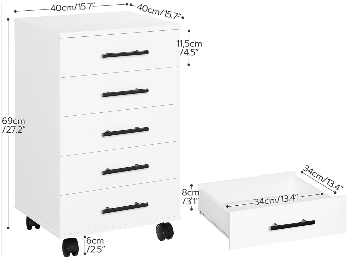
Image: Dimensional diagram of the HOOBRO 5-Drawer File Cabinet, including overall height, width, depth, and individual drawer dimensions.
