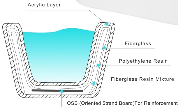
An illustrative cross-section revealing the bathtub's robust multi-layered construction, including acrylic, fiberglass, and OSB reinforcement.
