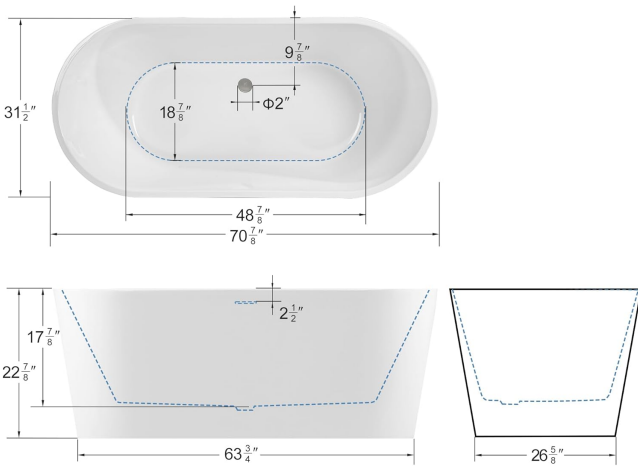
A detailed diagram outlining the precise dimensions of the bathtub, crucial for planning installation.
