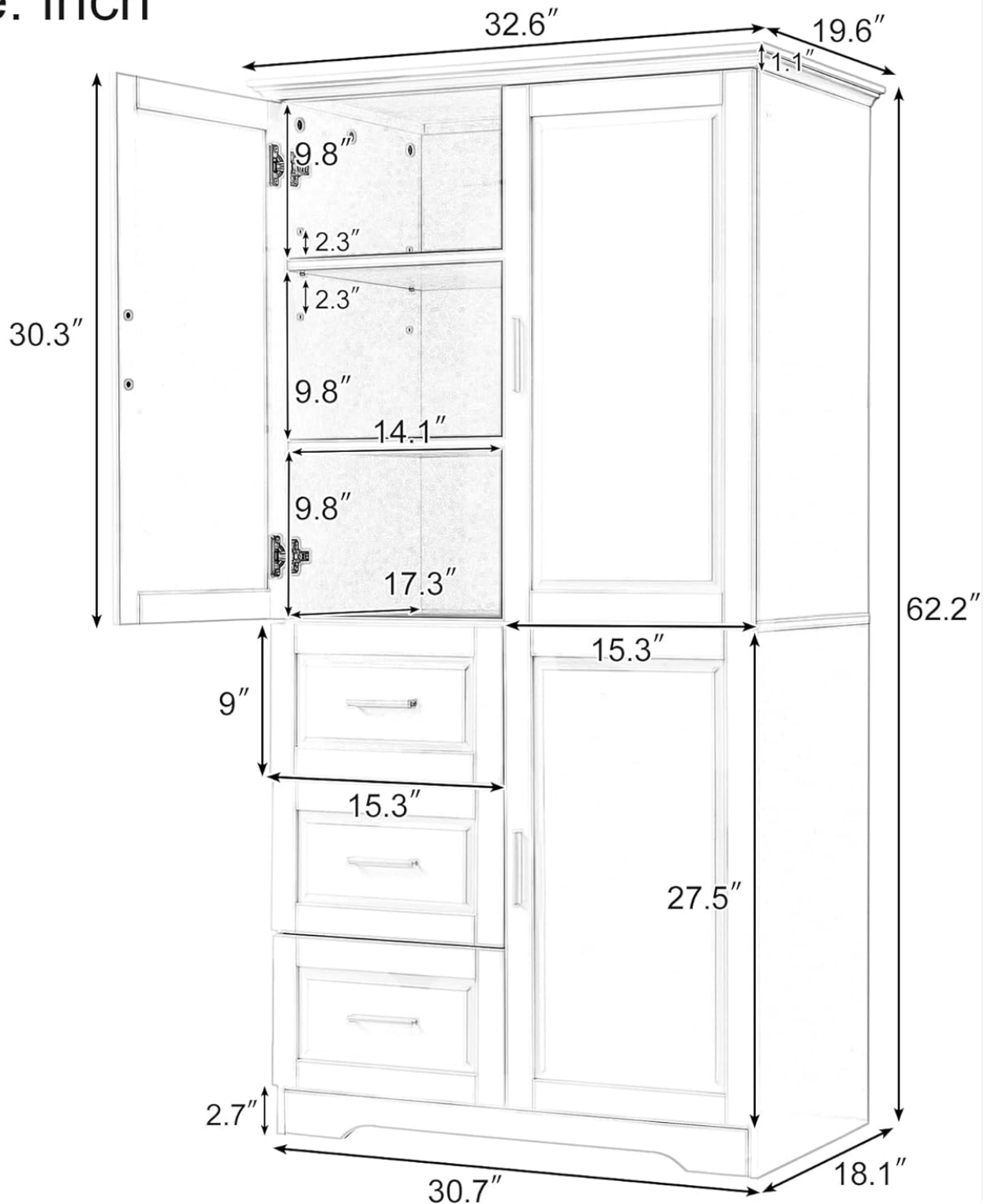
Image: A technical drawing providing precise dimensions of the Polibi Tall Storage Cabinet in inches, including height, width, depth, and internal measurements of shelves and drawers.
