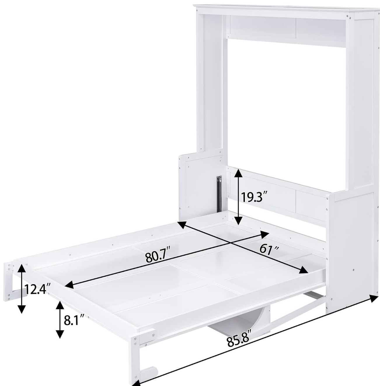
Image: Detailed dimensions of the Murphy Bed in its open configuration, including bed frame length, width, and height from the floor.
