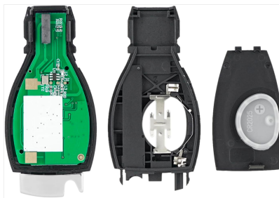
Figure 2.6: Close-up of the internal circuit board and the CR2025 battery compartment.
