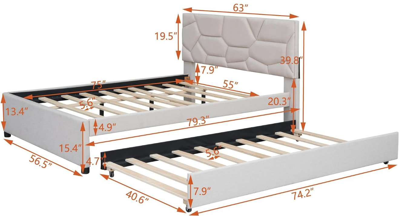
Figure 5: Detailed diagram showing the dimensions of the bed frame and trundle.
