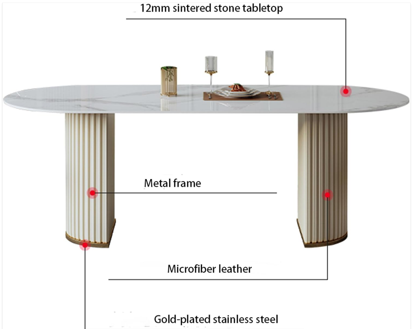
Figure 6.1: Detail of the sintered stone tabletop and microfiber leather leg.
