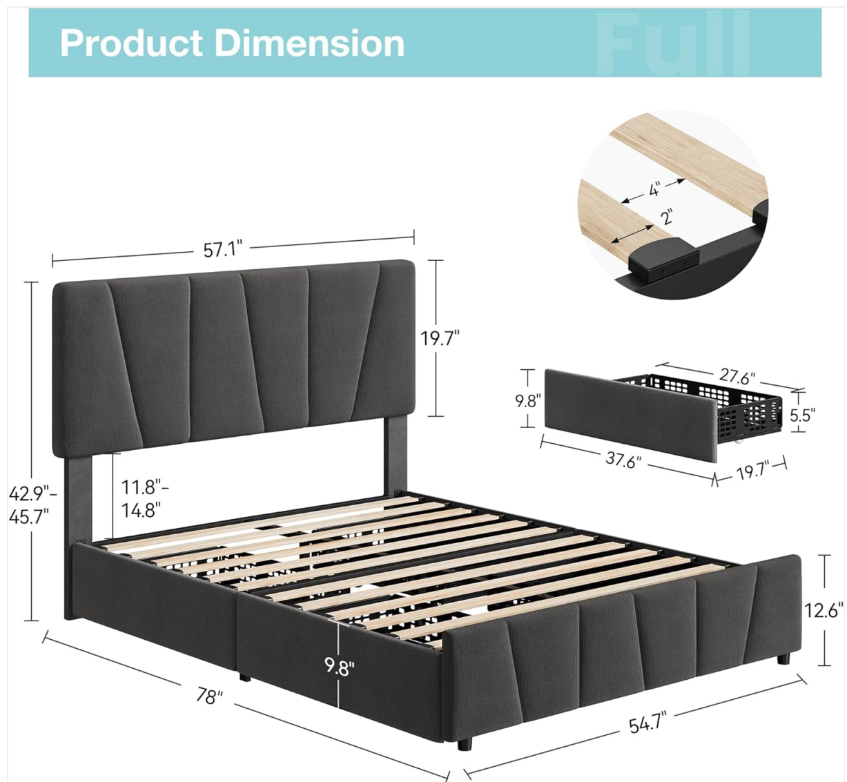
Image: Product dimensions diagram.
