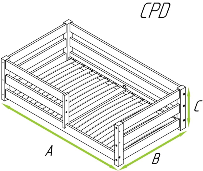
Image: Technical diagram illustrating the dimensions of the ADEKO CPD bed. It shows a length of 199 cm, a width of 141 cm, and a height of 44.7 cm, designed for a 135x190 cm mattress.
