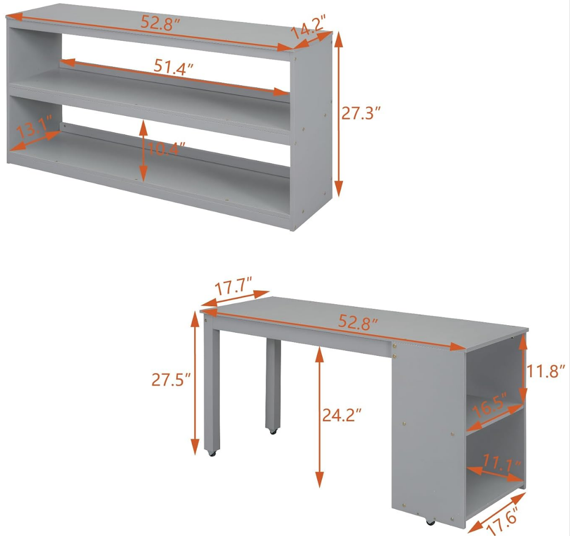
Figure 2: Retractable Desk Dimensions. This image provides detailed measurements for the desk component, including its length, width, and height, as well as the dimensions of its integrated shelves.
