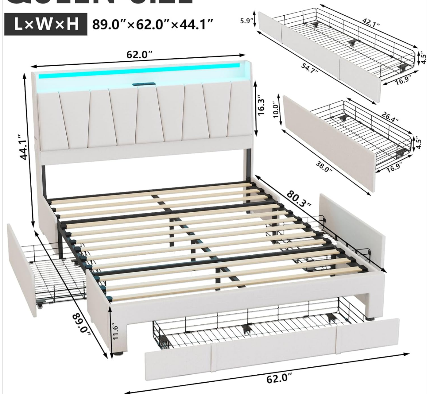
Figure 1: Queen Size Bed Frame Dimensions and Components. This diagram illustrates the overall dimensions of the bed frame (89.0"L x 62.0"W x 44.1"H) and provides a breakdown of its main parts, including the headboard, side rails, and the three storage drawers with their individual dimensions.
