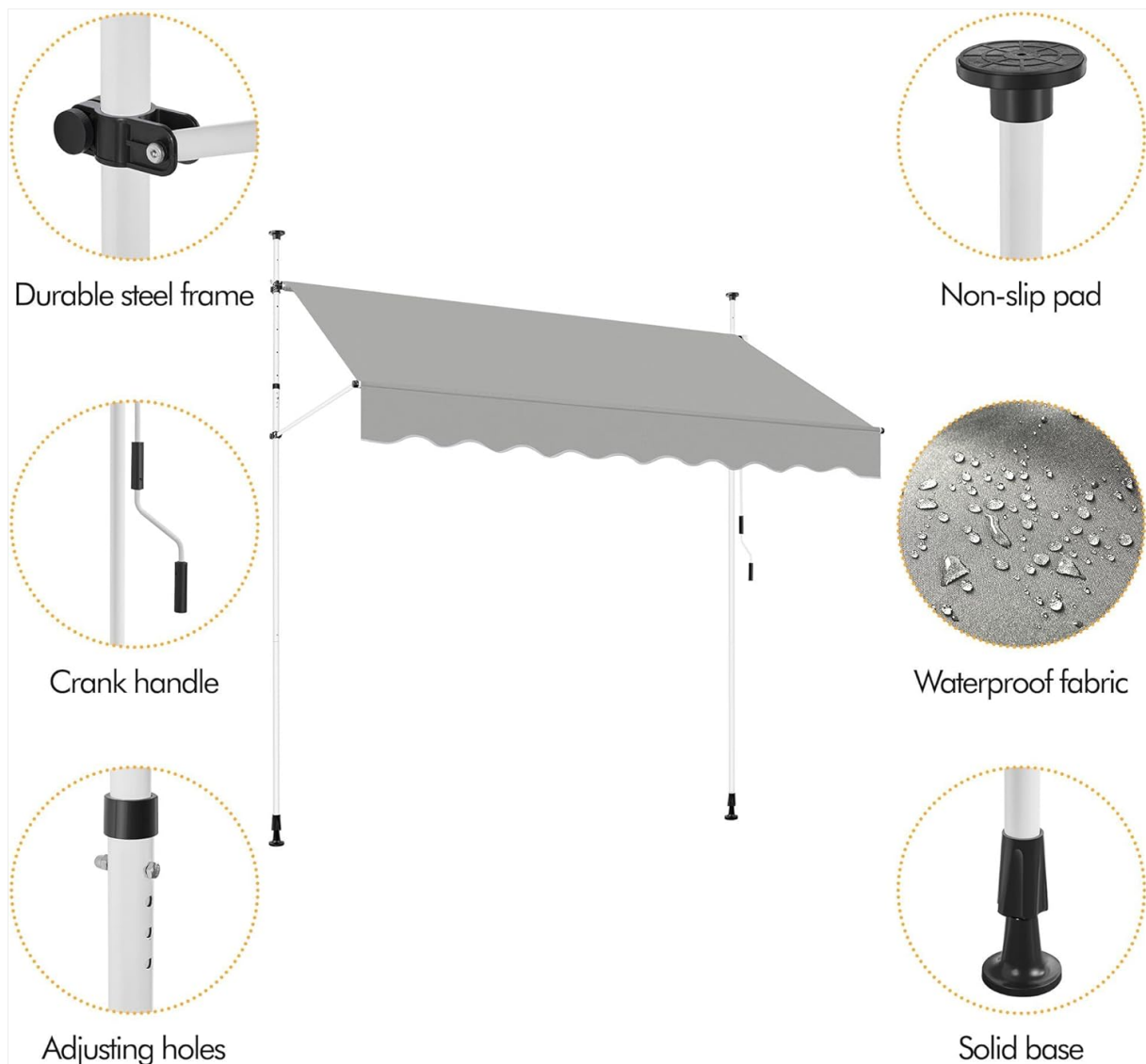
Figure 3.1: Key components of the Yaheetech Retractable Manual Awning.
