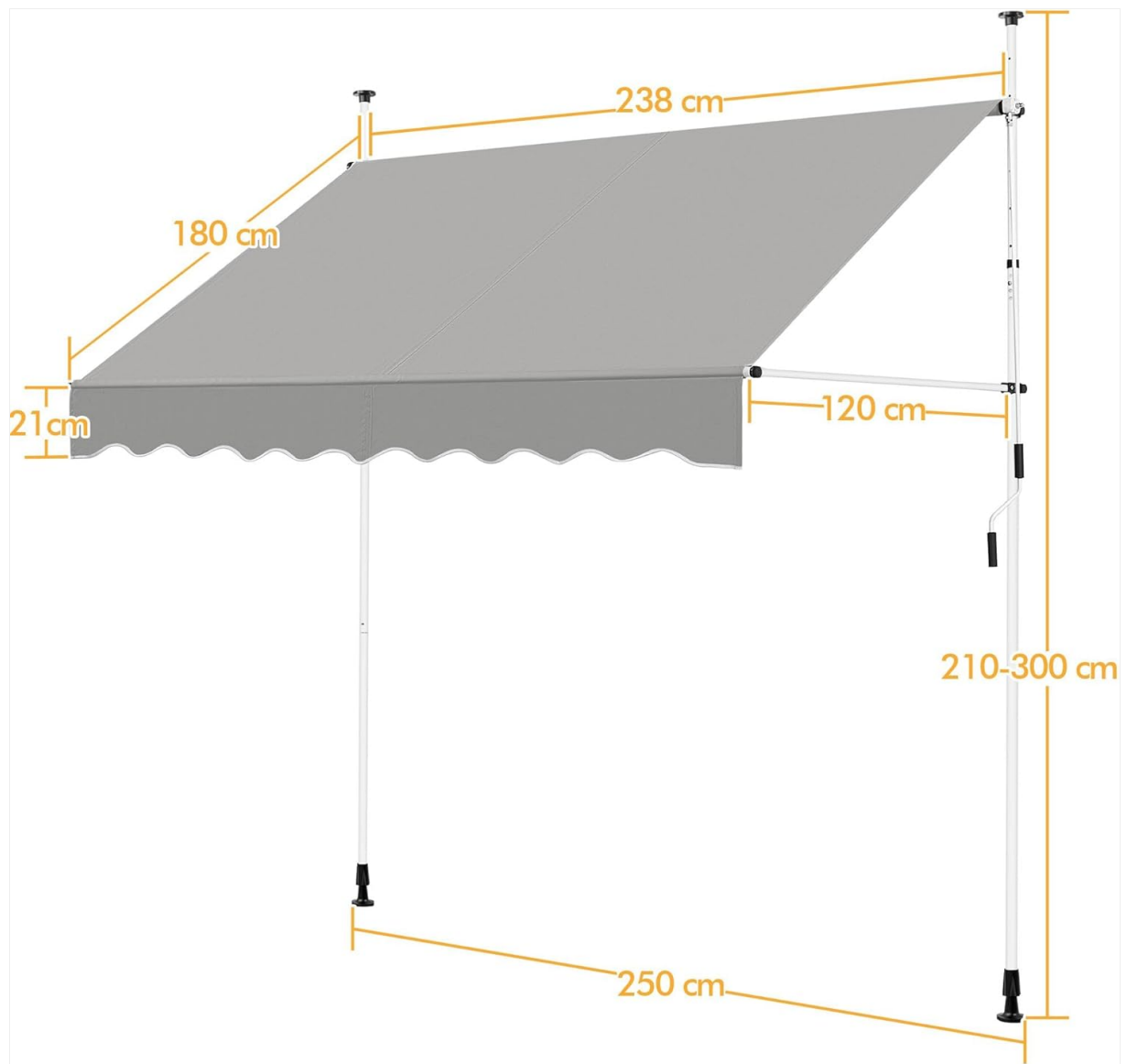
Figure 8.1: Dimensional overview of the awning.
