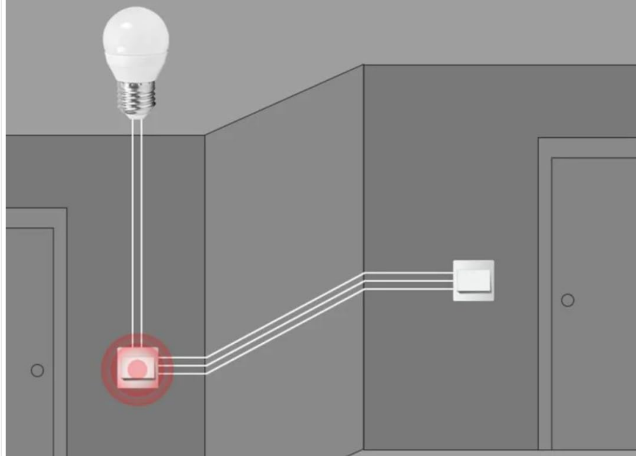
Figure 3: Wiring diagram for parallel connection, allowing the smart switch to work alongside a traditional switch.
