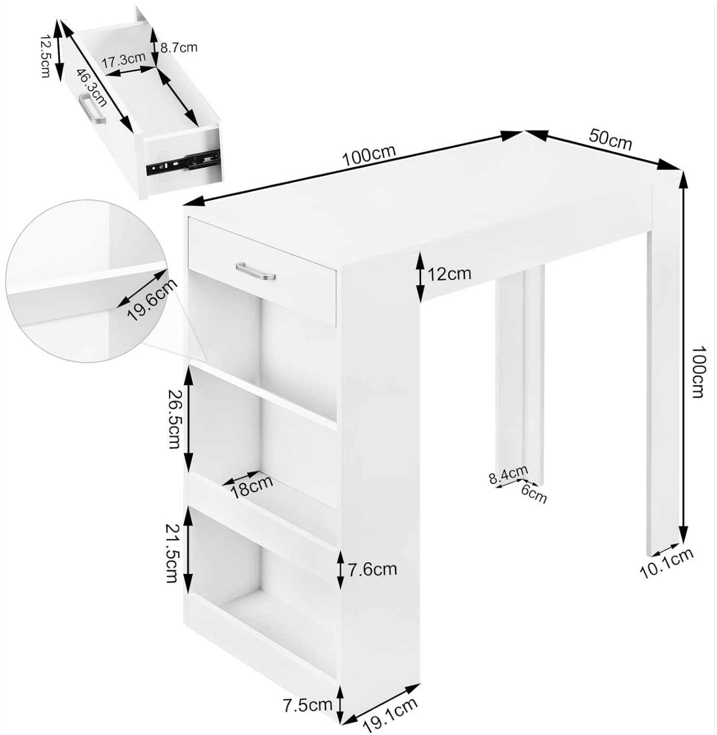
Image 4.1: Detailed dimensions of the bar table, including drawer and shelf measurements, crucial for assembly and placement.
