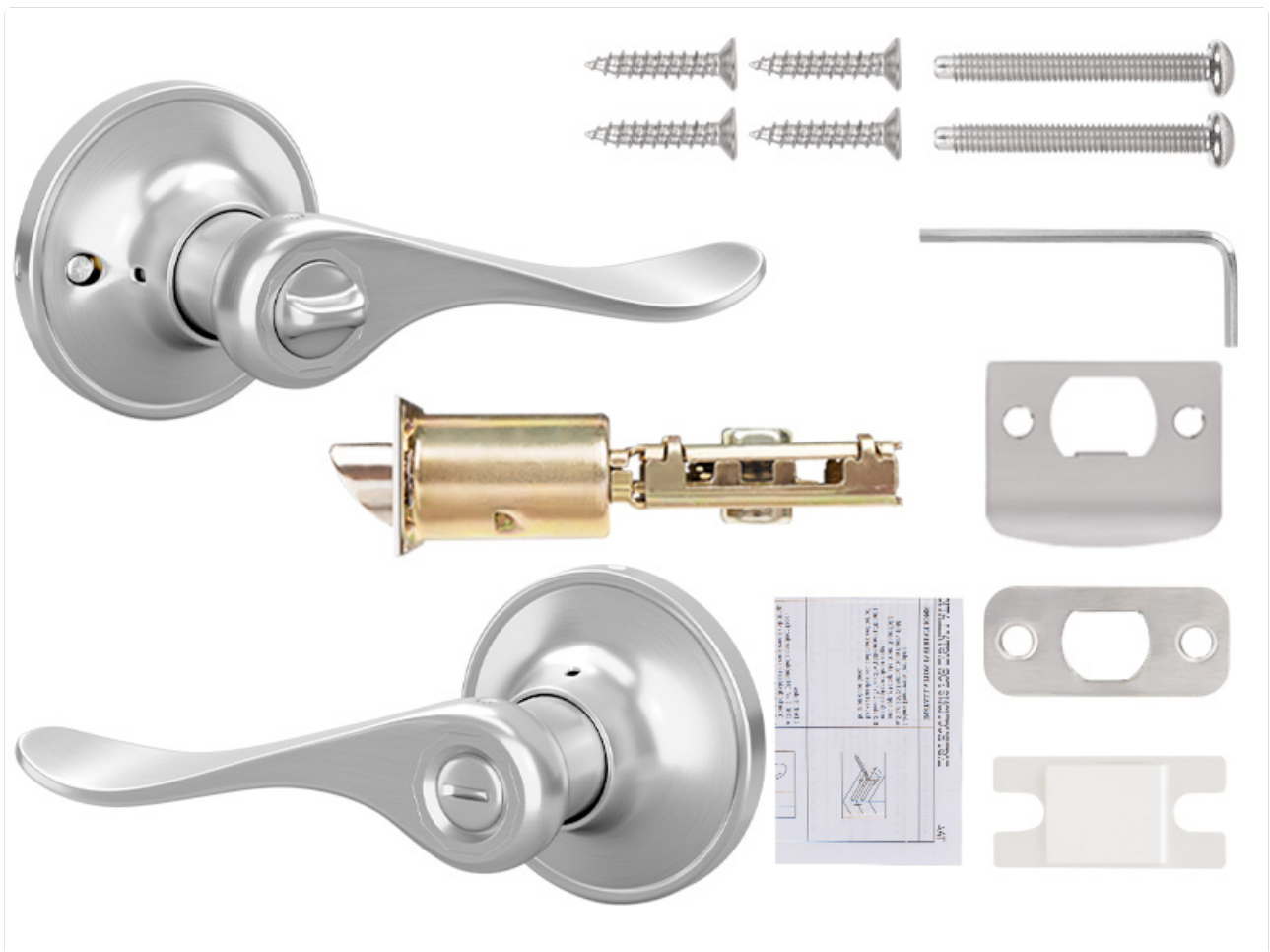
Image: An exploded view showing all parts included in the HOSOM door lever package, such as the levers, latch, strike plate, and screws.
