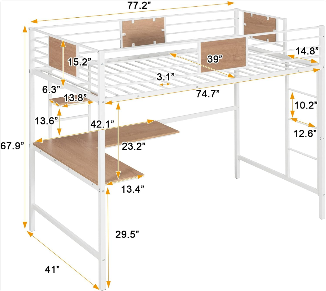
Figure 4: Comprehensive dimensions of the Twin Loft Bed.
