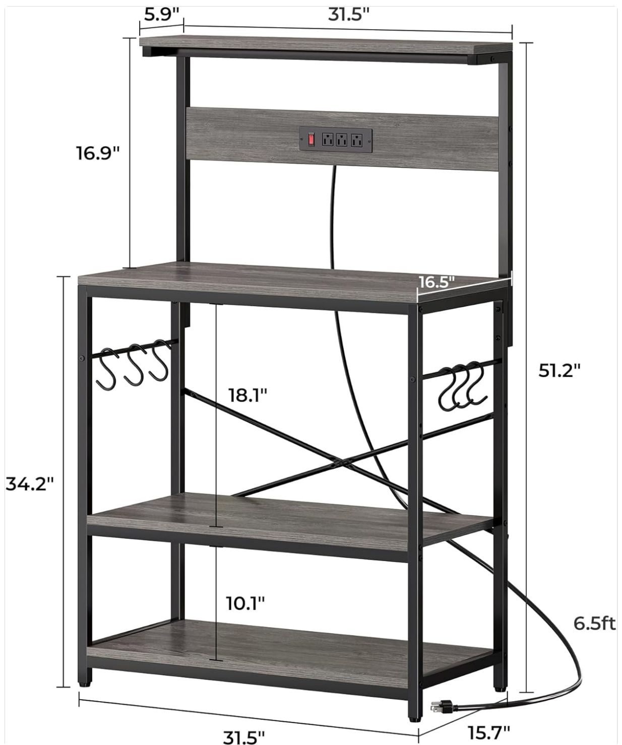
Image: A comprehensive diagram illustrating all key dimensions of the baker's rack, including height, width, depth, and shelf spacing.
