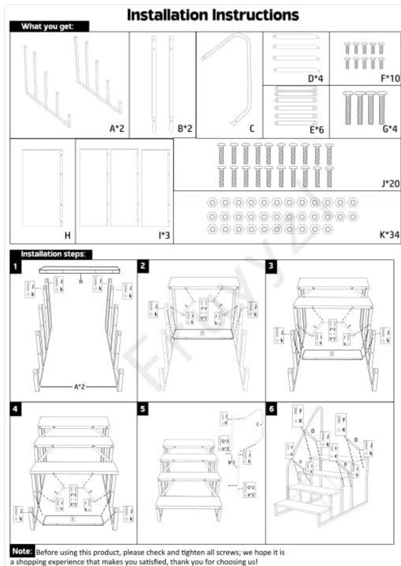
Figure 3: Installation Instructions Diagram.
