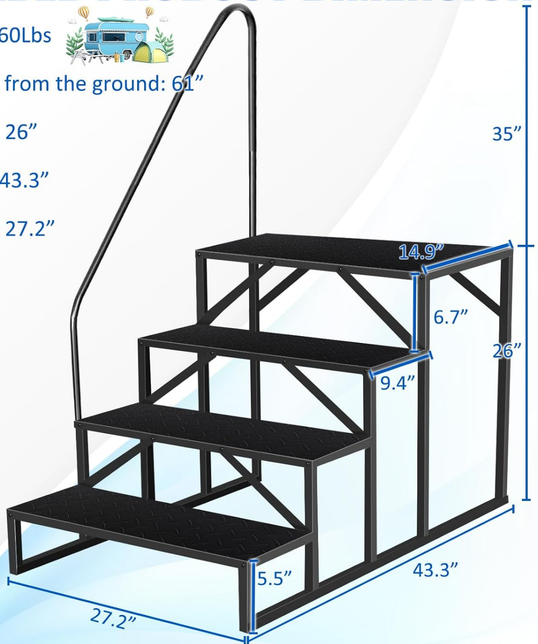
Figure 7: Product Dimensions and Load Capacity.
