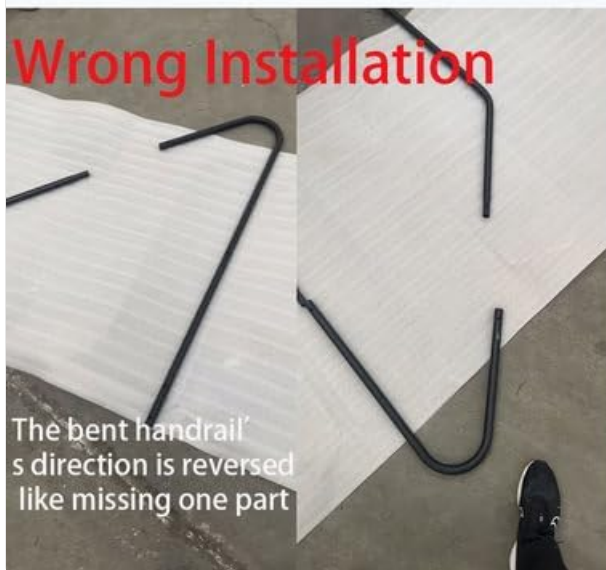
Figure 5: Handrail Installation Correction Guide.
