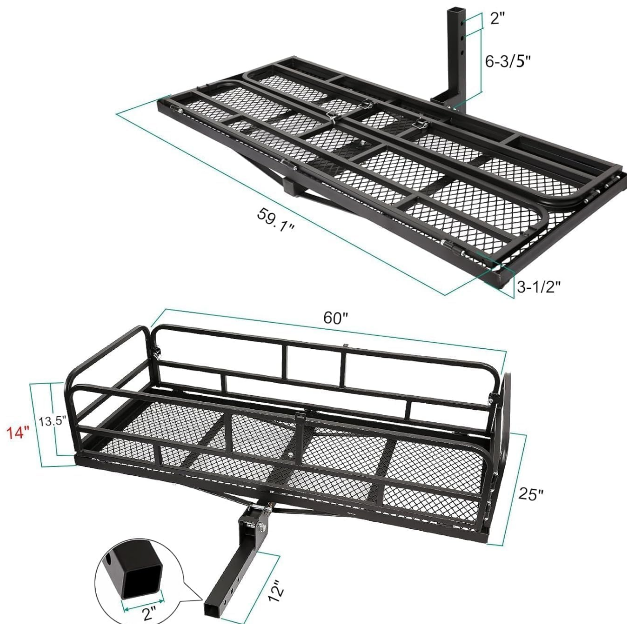
Figure 3: Detailed product dimensions.
