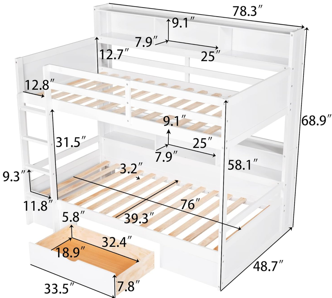
Figure 2: Detailed dimensions of the Polibi Twin Over Twin Bunk Bed, including overall length, width, height, and internal measurements for mattress placement and shelf depths.
