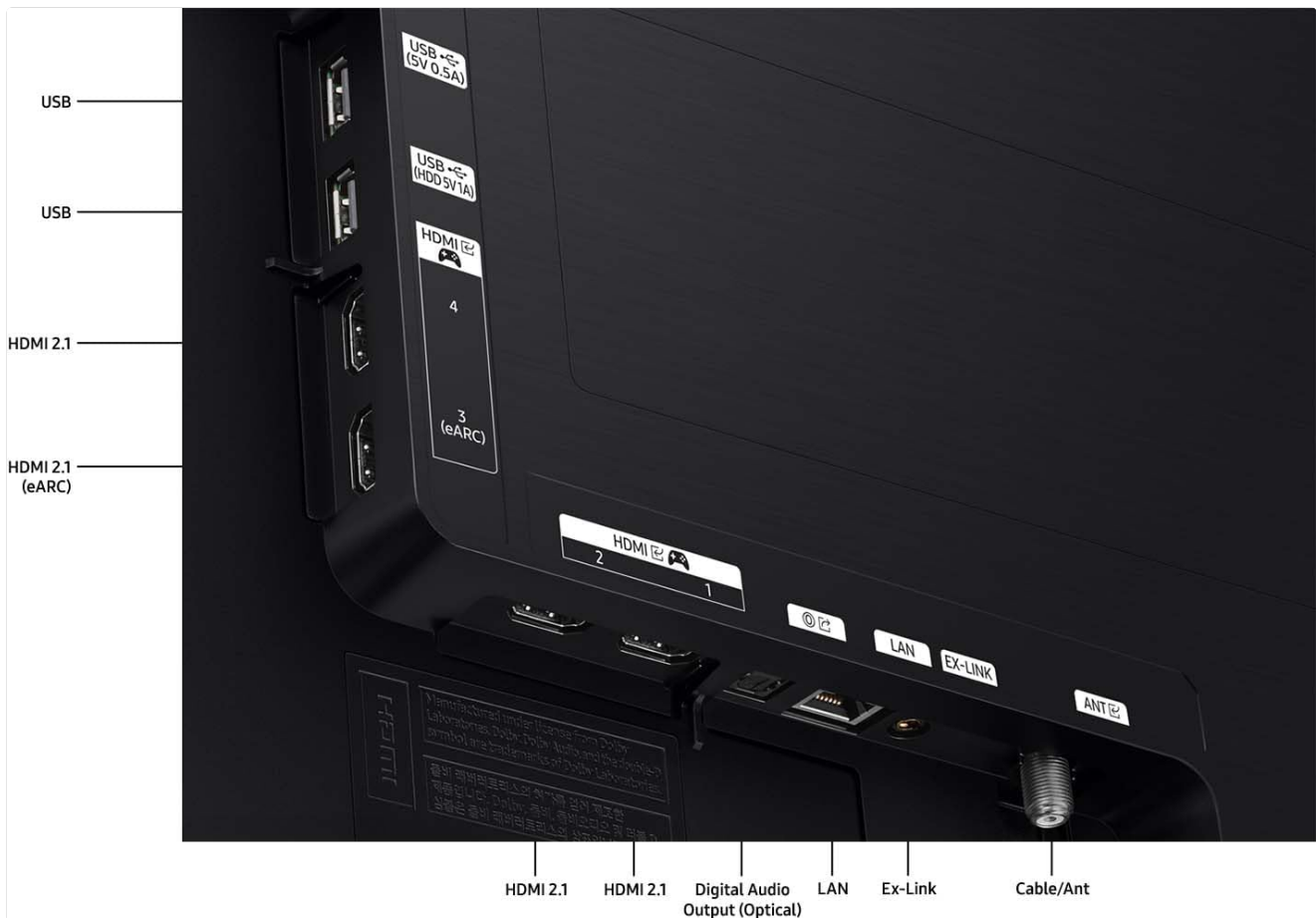
Figure 3.1: Rear view of the Samsung S95D TV's One Connect Box ports.
