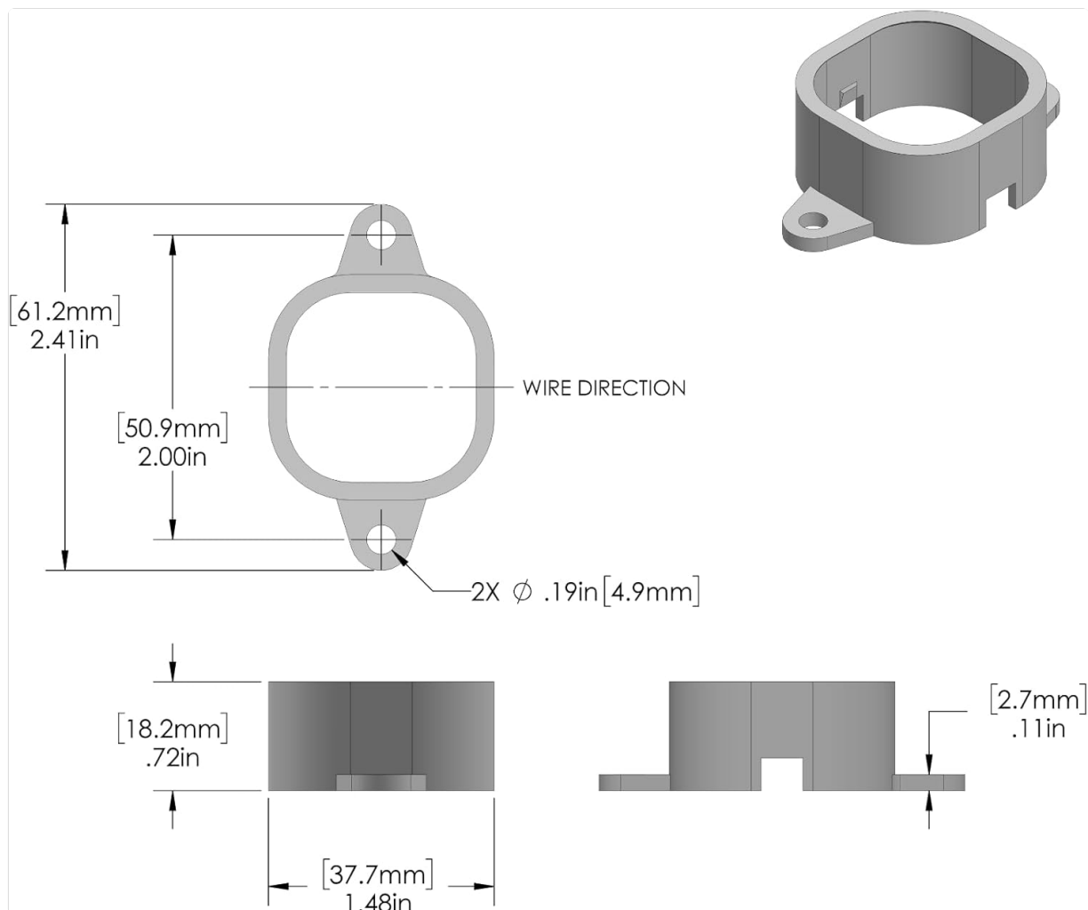
Figure 5: Mounting Bracket Dimensions.
